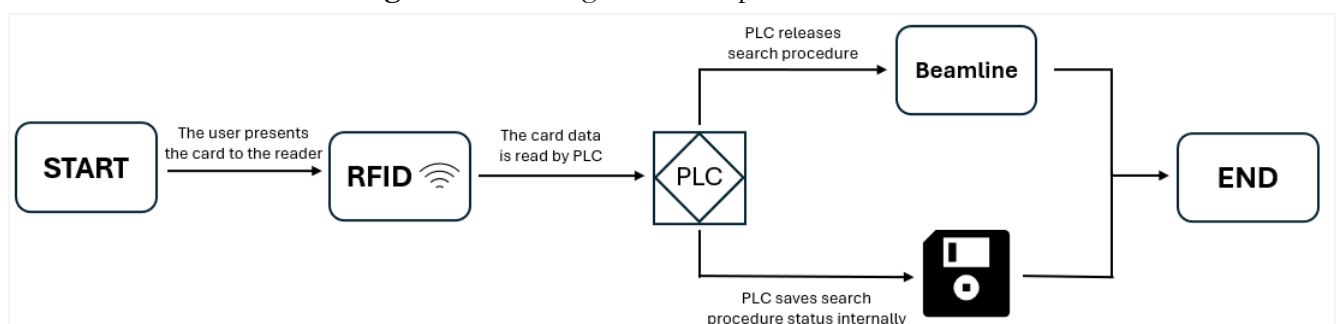
Figure 5: Enabling the search procedure for users
