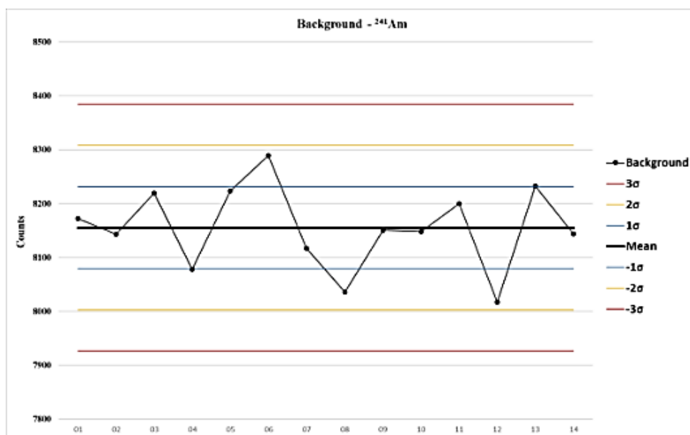
Figure 4: Background control charts for ^{241}\text{Am}
